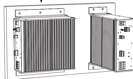
Figure 3. Wall and chassis mount
