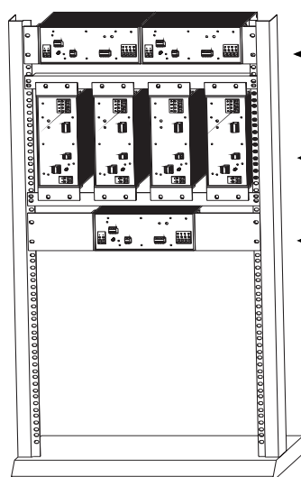
Figure 2. 19"-rack mounting
